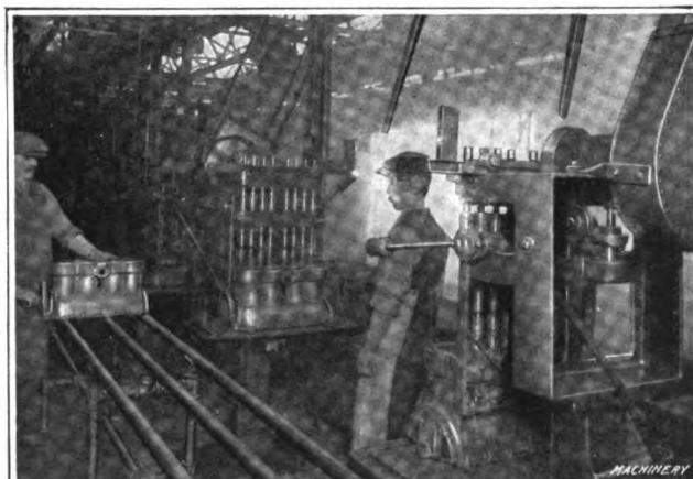
Fig. 17—For handling pieces that are too heavy to slide in troughs, and where it is only required to transport the work a short distance, rails are set up in the Ford Motor Co.'s factory, along which the work can be slid from machine to machine. This saves lost production during late hours of the afternoon which would otherwise be caused by machine operators becoming unduly fatigued
